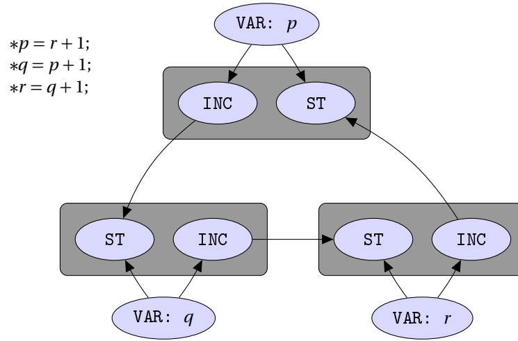
Fig. 19.5 DAG patterns may introduce cyclic data dependencies.
