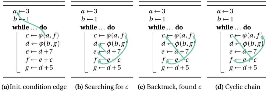
Fig. 10.1 Detection of the cyclic definition using a depth first search traversal of the use-def chains.
