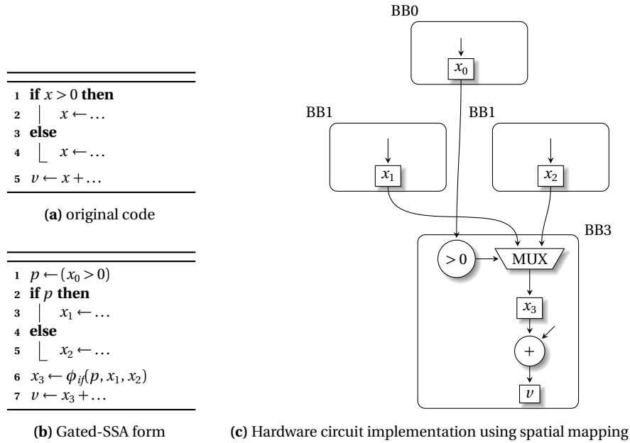
Fig. 23.5 Hardware generation example using Gated-SSA form
