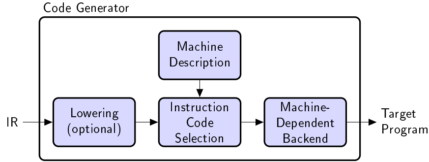
Fig. 19.1 Scenario: An instruction code selector translates a compiler's IR to a low-level machine-dependent representation.
