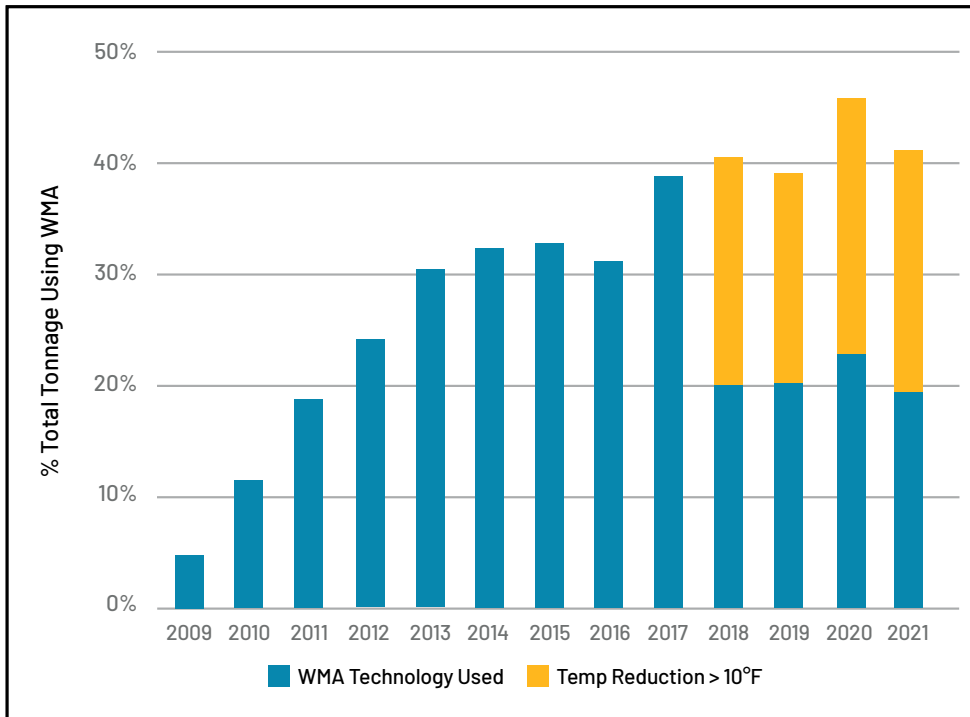
Figure 11. Percent of total tonnage produced using WMA technologies, 2009-2021. Data prior to 2018 did not differentiate between WMA production and WMA production with a temperature reduction. From Williams et al. (2022).
