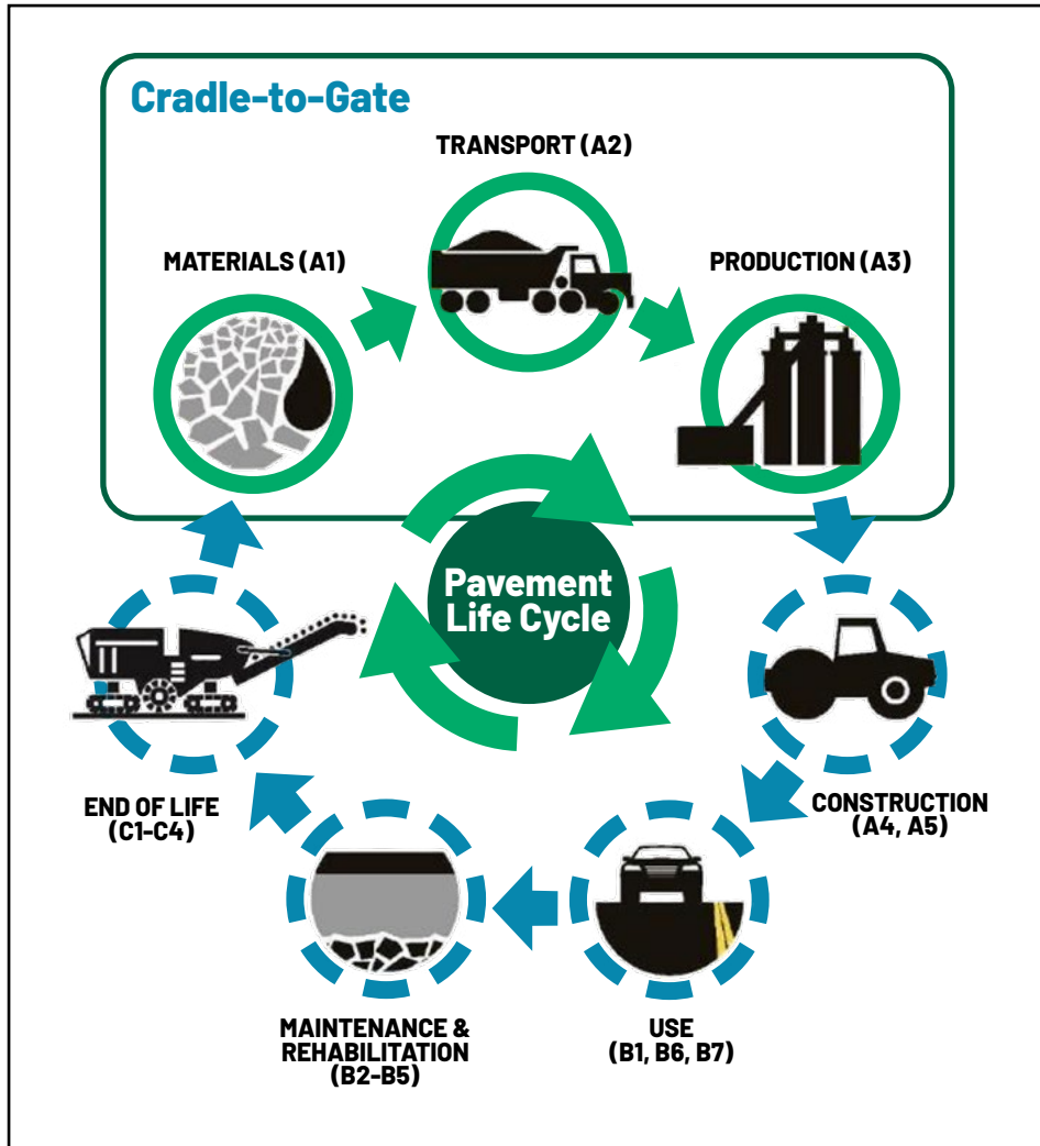
Figure 1. Key stages of the asphalt pavement life cycle with reference to the ISO 21930 life cycle information modules.
