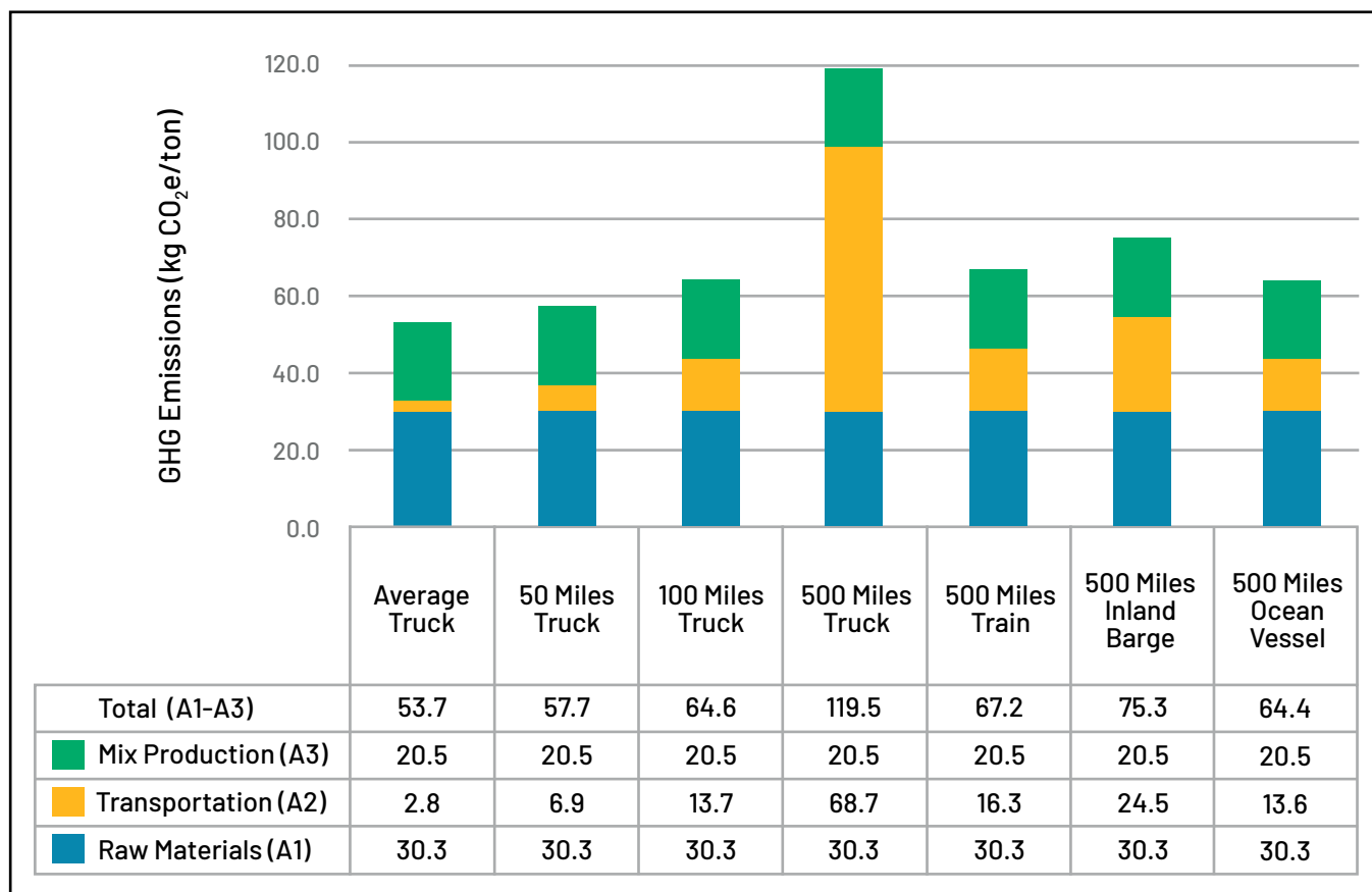
Figure 5. Impact of transport distance on transportation related (A2) GHG emissions. The Average Truck scenario assumes transport distances of 21.5 miles for aggregates and 3.9 miles for asphalt binder (Mukherjee, 2016). The sum of individual life cycle stages may not equal the total due to rounding effects.
