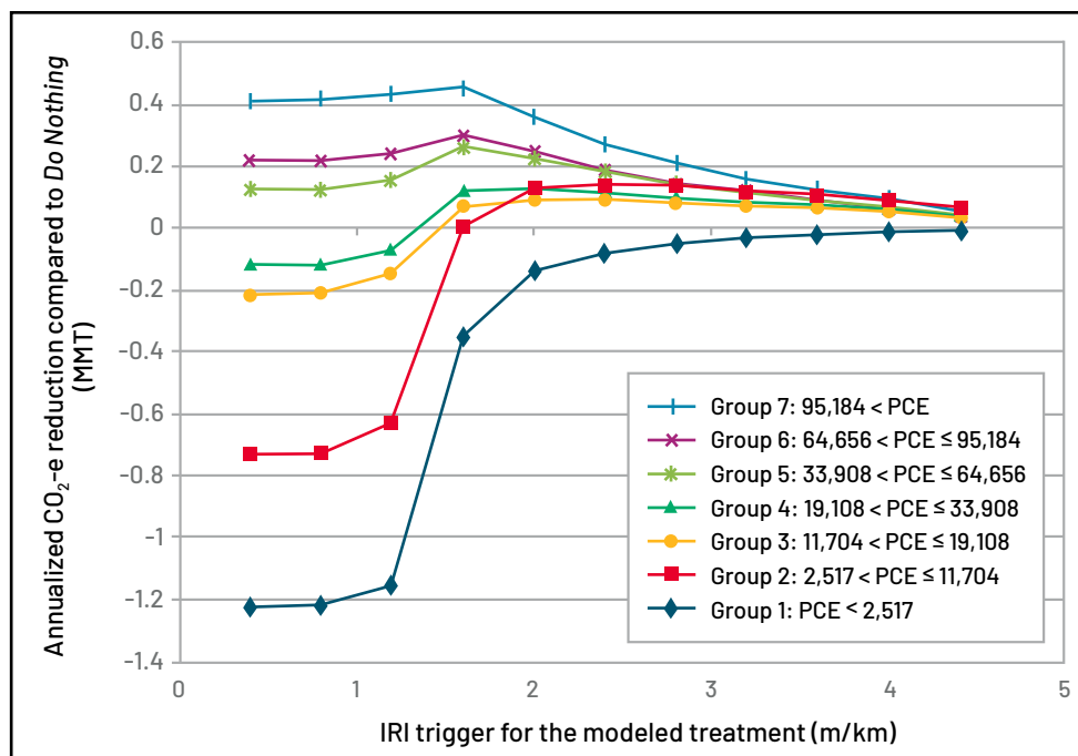
Figure 17. Annualized CO 2 e reductions versus IRI trigger for different traffic levels over a 10-year analysis period for the entire Caltrans pavement network compared to maintaining the network at approximately its current roughness and macrotexture. The optimal IRI trigger is lower for high volume roads. Low volume roads (Group 1) never achieve a net GHG emission reduction. PCE is daily passenger car equivalents. From Wang et al. (2014b).
