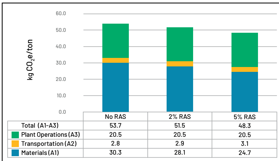
Figure 9. Impact of RAS on cradle-to-gate (A1-A3) emissions of an asphalt mixture. Total asphalt binder content for each mix is 5%. RAS is assumed to have a 20% asphalt binder content and to offset the virgin binder content accordingly (e.g., a mix with 5% RAS would have a virgin binder content of 4% and a recycled binder content of 1%). Units in the data table are in kg CO 2 e/ton of mix. The sum of individual life cycle stages may not equal the total due to rounding effects.
