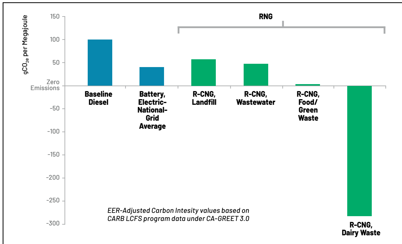
Figure 13. Life cycle carbon intensity (CI) values for CNG as a transportation fuel sourced from renewable sources (R-CNG). R-CNG feedstocks have low or even negative CI scores because they capture emissions that would otherwise be released to the atmosphere. From NGVAmerica (2019).
