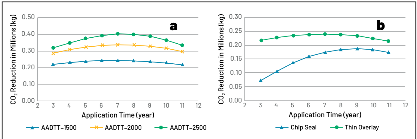
Figure 18. (a) Net CO 2 emission reductions for different AADTT values and application times in the production, construction, and use stages of Thinlays. (b) Comparison of net CO 2 reductions for Thinlays and chip seals with AADTT of 1500 ESALs. For both graphs, Initial IRI = 1.0 m/km. For each point, the analysis was conducted for one lane-mile of asphalt pavement with a speed limit of 65 mph from application of the thin overlay until IRI reached a terminal value of 2.714 m/km. The inflection point in each AADTT curve represents the optimal application time for achieving net CO 2 reductions. From Wang et al. (2019).
