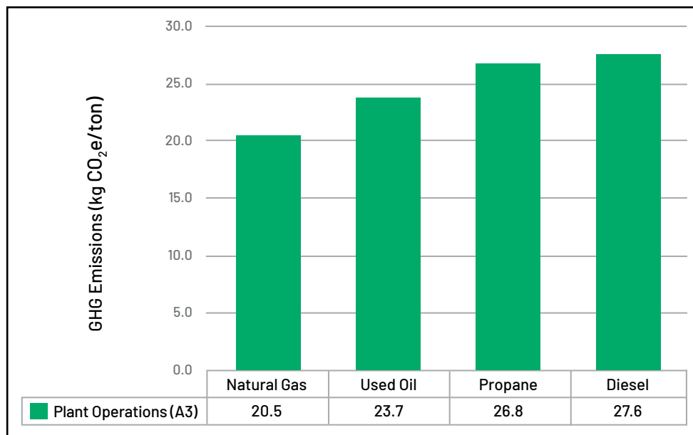
Figure 12. GHG emissions from plant operations (A3) for asphalt mixtures produced using various fuels on an equivalent Btu basis.
