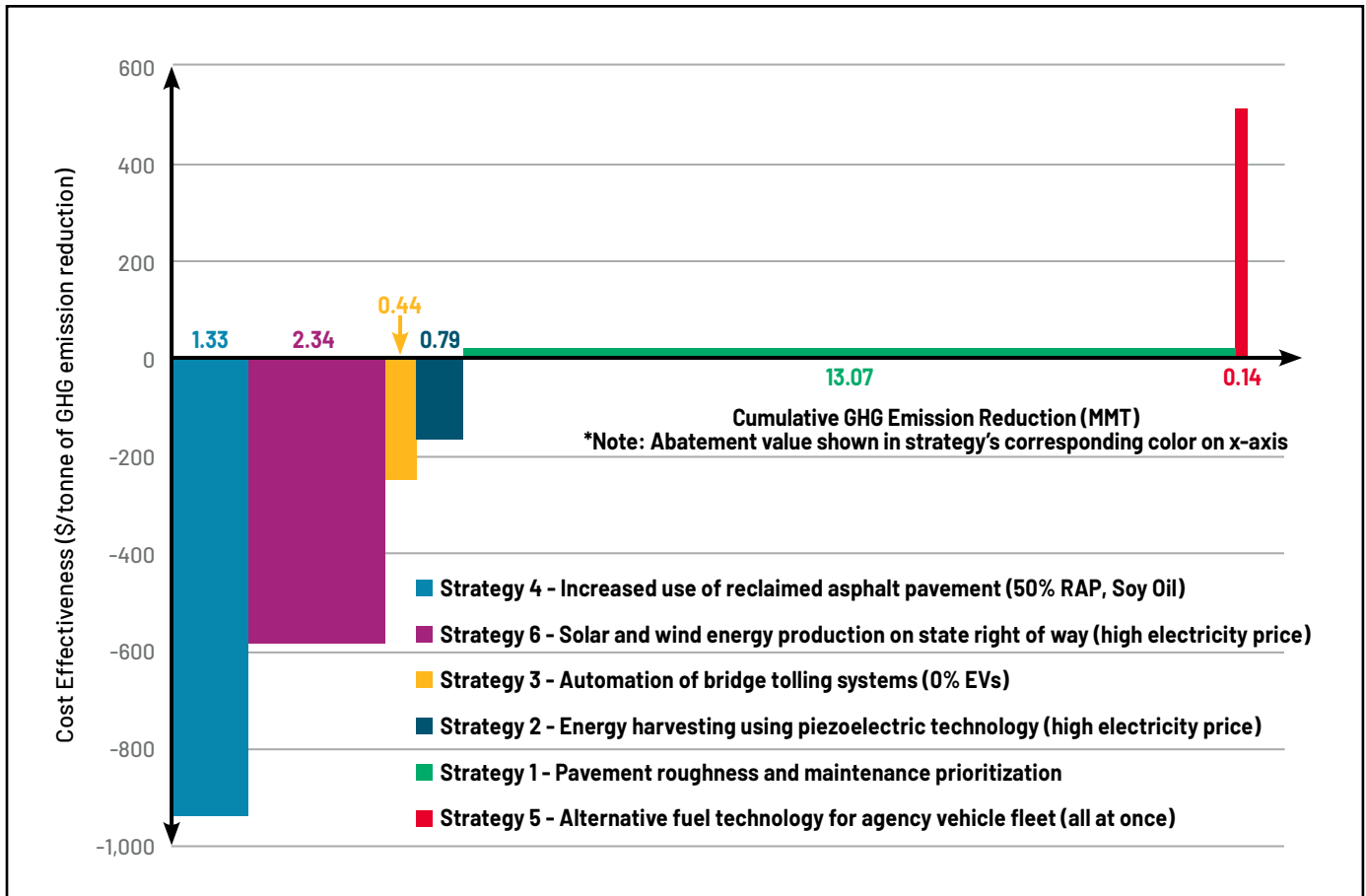
Figure 19. Supply curve for six pilot case studies for optimistic scenarios considering both GHG and cost-effectiveness. Strategy 4, increased use of RAP, was the most cost effective. Strategy 1, pavement roughness and maintenance prioritization, had the greatest cumulative GHG emission reduction potential with 13.07 MMT CO 2 e. Emission reductions for Strategy 1 represent the overall Caltrans pavement network over a 35-year analysis period. From Harvey et al. (2019).
