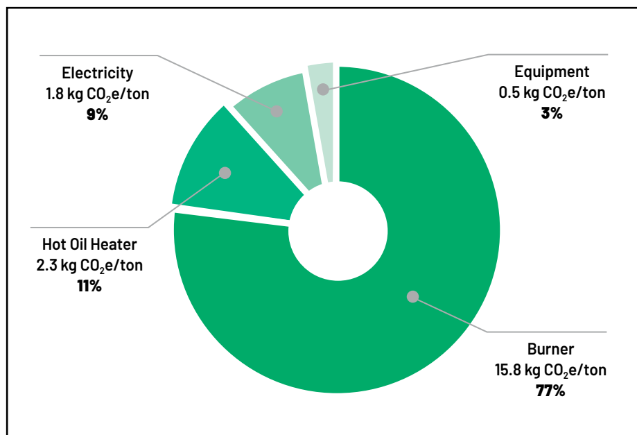
Figure 6. Mix production related GHG emissions (A3) for a typical asphalt plant with grid-supplied electricity that consumes natural gas for the burner and hot oil heater and diesel fuel for mobile equipment. Data inputs are provided in Appendix A. The sum of individual unit processes does not equal the A3 total of 20.5 due to rounding effects.
