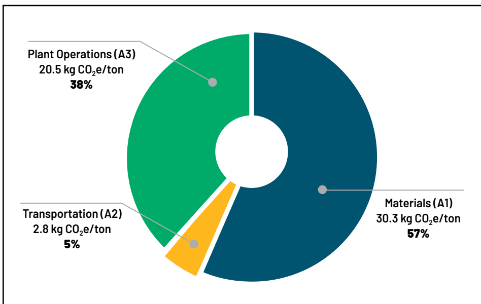
Figure 3. Cradle-to-gate GHG emissions (A1-A3) for the baseline reference scenario, which is a typical asphalt mixture with no recycled materials and average transportation distances produced at a plant that burns natural gas. The sum of individual life cycle stages does not equal the total of 53.7 due to rounding effects.
