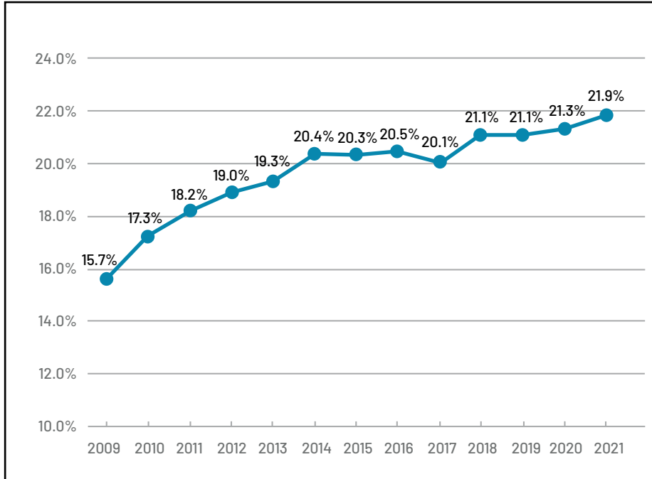
Figure 8. Average RAP content of new asphalt mixtures, 2009-2021. From the IS-138 series (e.g., Williams et al. 2022).
