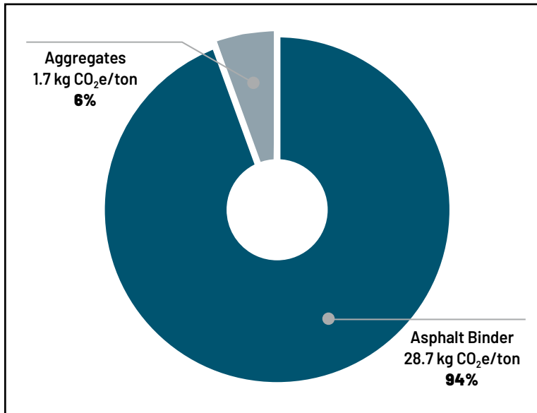
Figure 4. GHG emissions during upstream production of raw materials (A1) for a typical virgin asphalt mixture that contains 95% aggregates and 5% asphalt binder. The sum of individual materials does not equal the A1 total of 30.3 due to rounding effects.
