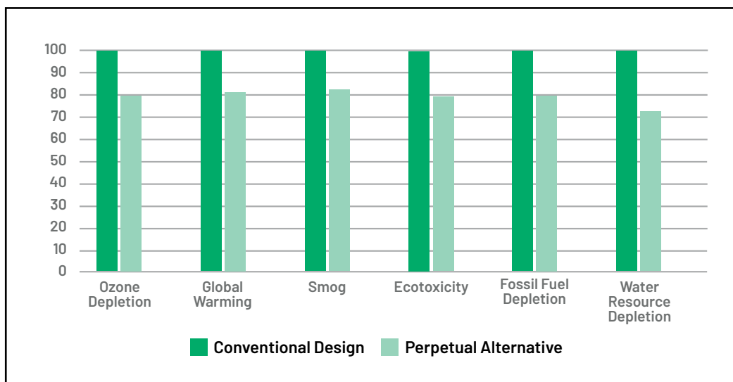
Figure 16. LCA results for a conventional design and perpetual alternative for an Iowa highway over a 50-year analysis period. Values for the conventional design were established as the baseline, set at 100 percent. From FHWA (2020d).
