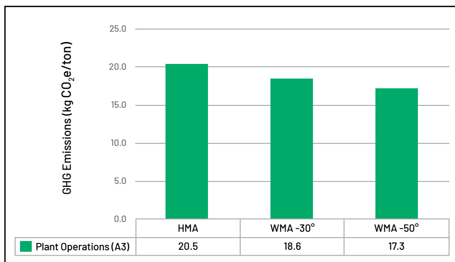
Figure 10. Potential reductions in GHG emissions from use of WMA technologies to reduce mix production temperature. HMA is hot-mix asphalt produced at a typical plant using natural gas for the baseline reference scenario presented in Section 2.1. WMA scenarios assume a reduction in burner fuel consumption of 1,000 Btu/°F/ton.
