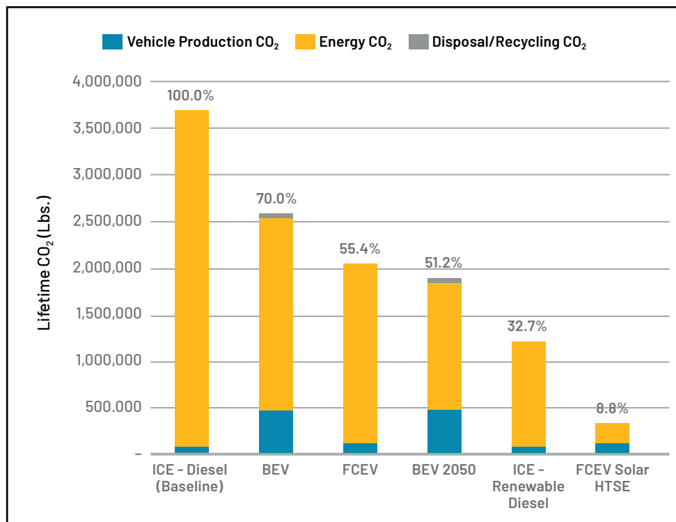
Figure 14. Scenario analysis of life cycle GHG emissions for various heavy-duty vehicle technologies. ICE is internal combustion engine, BEV is battery electric vehicle, BEV 2050 uses the Energy Information Administration (EIA) projected grid mix of energy supply for the year 2050, FCEV is fuel cell electric vehicle, and FCEV Solar HTSE assumes that the hydrogen is generated using solar powered high-temperature steam electrolysis. From ATRI (2022).
